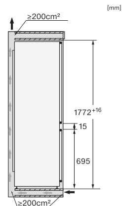
KFN7795D, side view (installation drawings)
