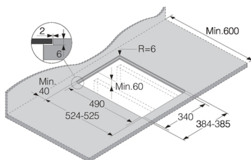
Flush built
