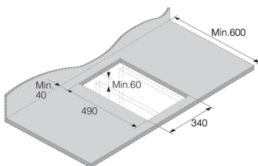
Top built
