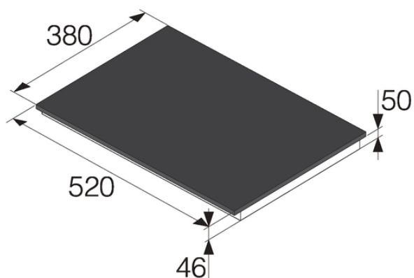
Top built
